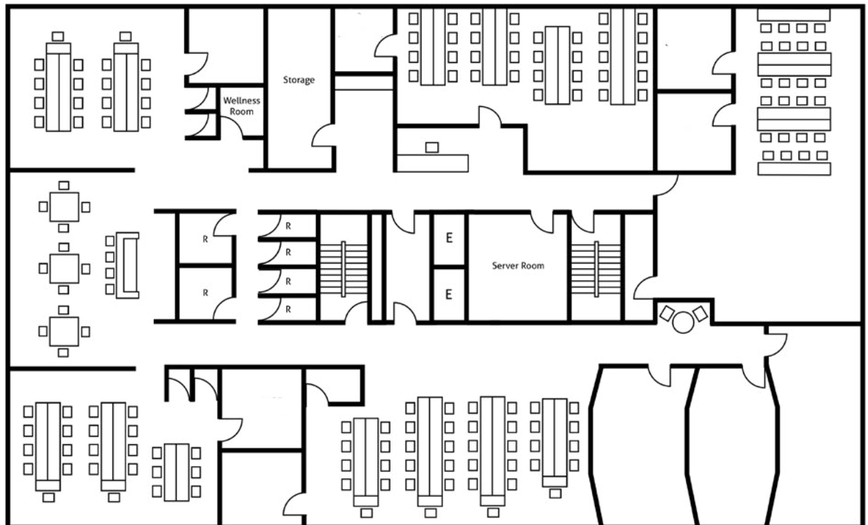
4 th Floor
