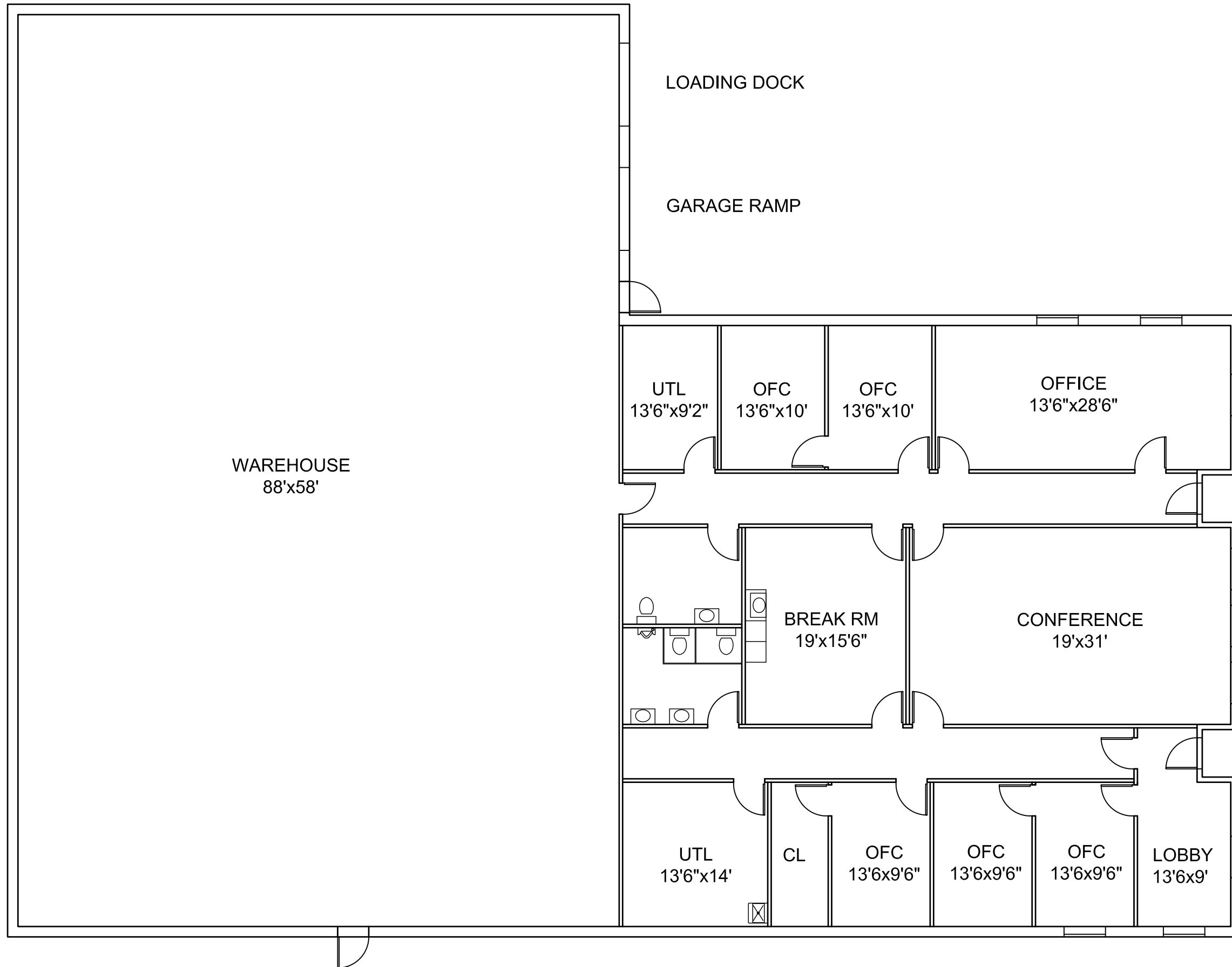
615 J AVE BUILDING LAYOUT
