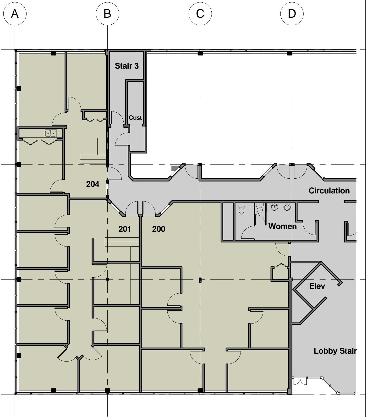
① Suites 3-200, 201, 204 3/32" = 1'-0"
